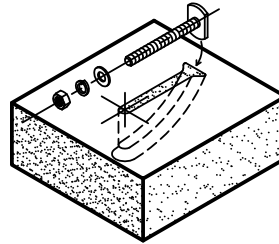
T-31 BACK ANCHOR
